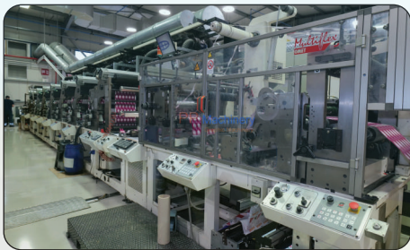
Omet Multiflex F-420 (8 Colors)
